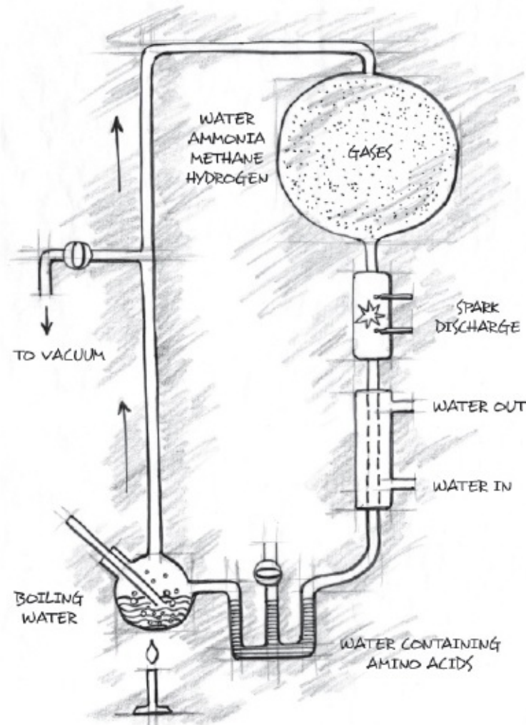
Figure 2.5. The Miller-Urey experiment.
