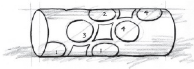
Figure 5.1. A simplified version of George Gamow’s own drawing depicting his direct template model of protein synthesis. The diamonds represent places where he thought various twenty amino acids would bond to the DNA double helix. The circles represent one of the four nucleotide bases. Gamow thought that the amino acids would nestle into the grooves between the nucleotide bases and that the structure of the DNA molecule would somehow determine where individual amino acids would bond, thereby directly determining protein sequencing.
