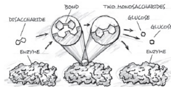
Figure 4.4. An enzyme ( \beta -D-galactosidase) breaking apart a two-part sugar molecule (a disaccharide). Notice the tight three-dimensional specificity of fit between the enzyme and the disaccharide at the active site where the reaction takes place. Notice also that the active site is small in relation to the size of the enzyme as a whole.
