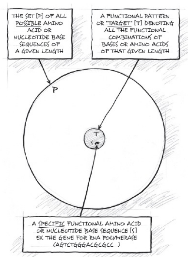
Figure 16.3. A functionally specified sequence of nucleotide bases or amino
