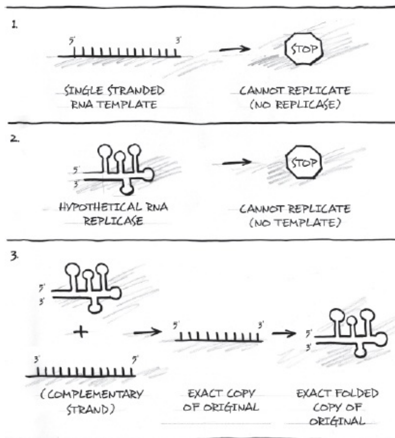
Figure 14.6. The minimal requirements for template-directed RNA self-replication as envisioned by Joyce and Orgel. They insist that any RNA
